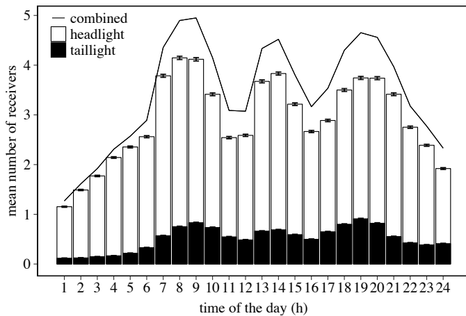
Figure 2. Mean number of receivers of a V-VLC transmission differentiated by the transmitting light module. The error bars (often indistinguishable due to their small size) indicate the 95 % confidence interval.
